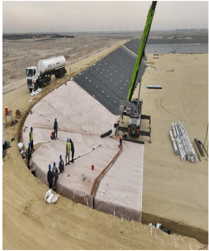
Geosynthetic Lining works at Soil Remediation Project
